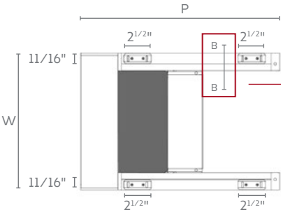
Rear view
