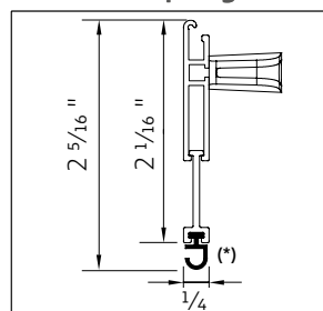
Extended spring
