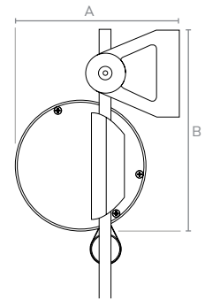
Ø12 rod guide adjustable fixing
