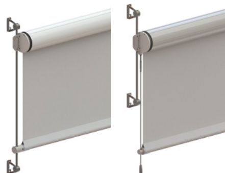
Special fixing configurations
