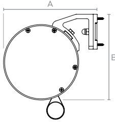
Wall short bracket
