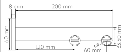
Rail Dike double
