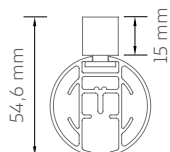
Rail Aeris plafond
