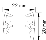
CLOSURE BOTTOM BAR
