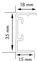
"A1" SIDE CHANNEL
