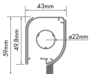
CASSETTE
