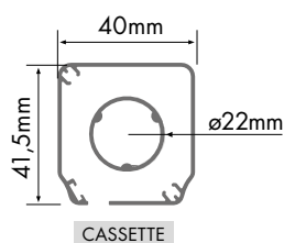
CASSETTE
