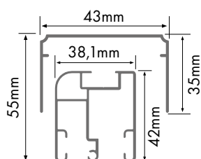
UPPER RAIL
