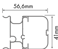
HANDLE BAR
