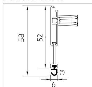
EXTENDED SPRING
