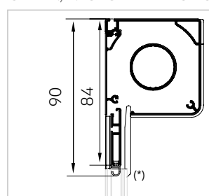
CHAIN/MOTOR RETRACTION HEIGHT
